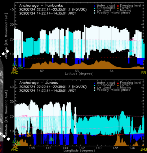
Cloud Vertical Cross-section [kft]
