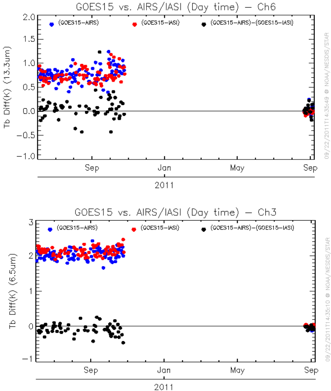
Figure 4.33: Comparisons of the GOES-15 band-6 (top panel) and band-3 (lower panel) before (left hand side) and after (right hand side) after the spectral response shift was implemented.
