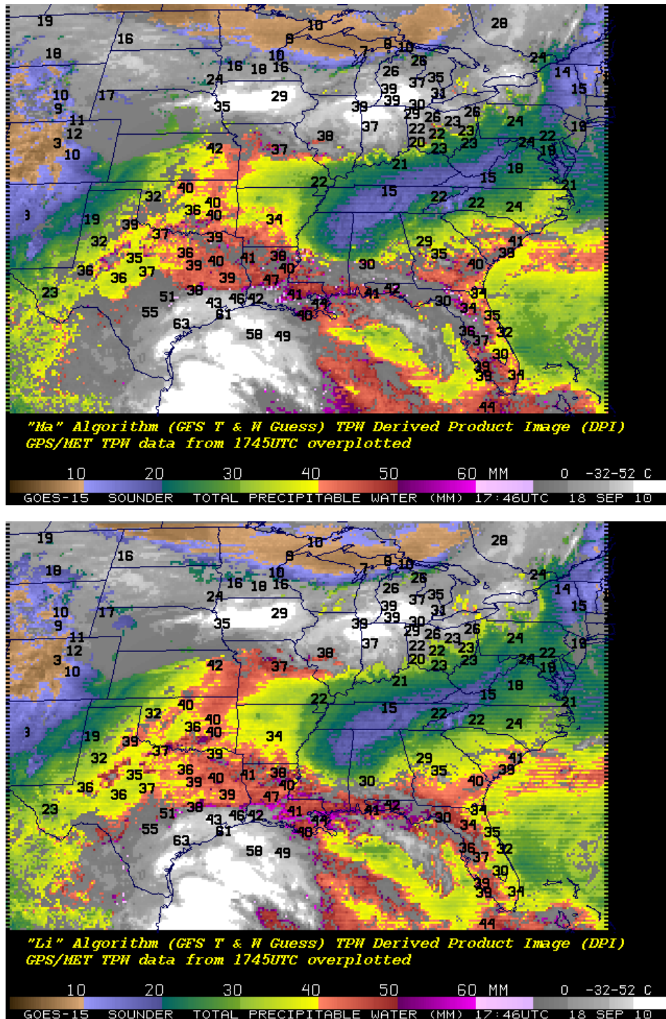
Figure 5.6: GOES-15 Sounder TPW from two retrieval algorithms (i.e., “Ma” (upper-panel) and “Li” (lower-panel)). Both images are from 18 September 2010.
