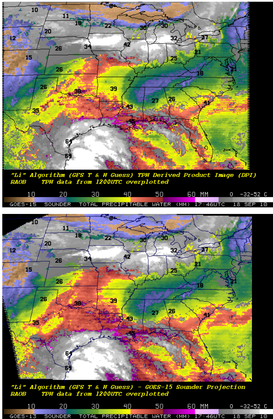
Figure 5.5: GOES-15 (top panel) and GOES-13 (lower panel) retrieved TPW (mm) from the Sounder displayed as an image. Cloudy FOVs are denoted as shades of gray. The data are from 1800 UTC on 18 September 2010. Measurements from RAOBs are overlaid text.
