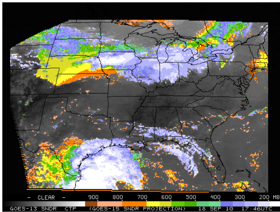
Figure 5.10: GOES-13 cloud-top pressure from the Sounder from 1746 UTC on 18 September 2010.
