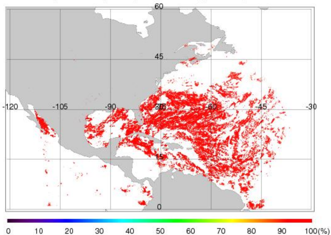
Figure 5.16: The nighttime areas that are considered clear pixels based on Bayesian estimate of \geq 98\% clear sky probability. The mask is based on the highest clear sky probability for the three daytime images that went into generating this GOES-15 product.
