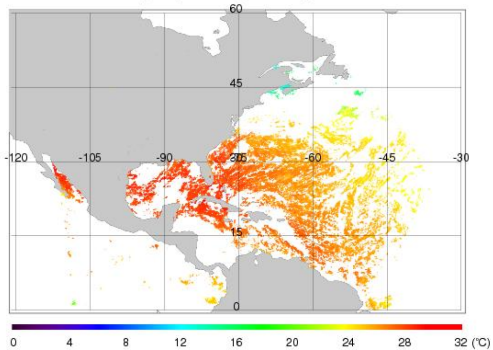
Figure 5.18: The SST from GOES-15 created by compositing three nighttime half hour SST McIDAS Area files with an applied threshold of \geq 98\% clear sky probability.
