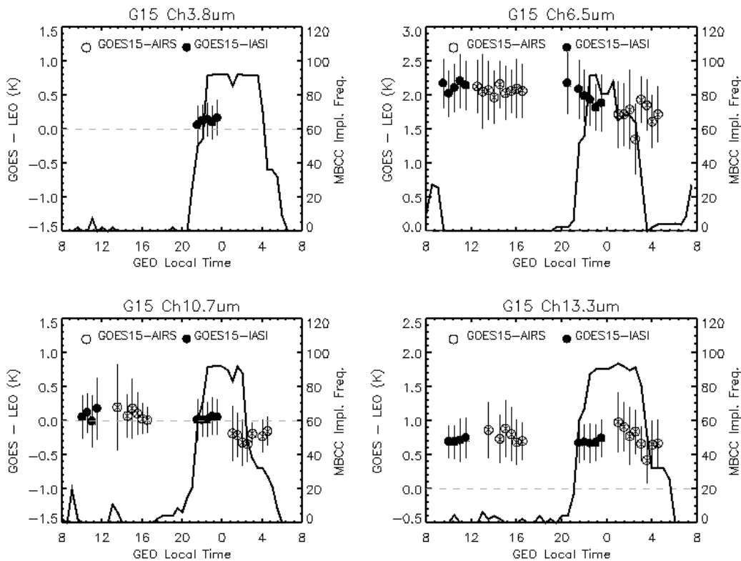
Figure 4.23: The Mean Tb bias to AIRS/IASI for GOES-15 Imager IR bands.
