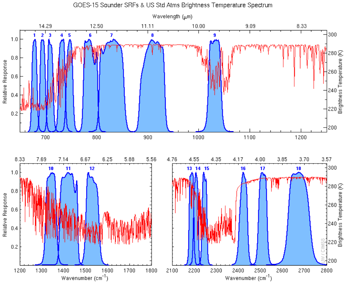
Figure 4.8: The eighteen GOES-15 Sounder IR-band SRFs super-imposed over the calculated high-resolution earth-emitted U.S. Standard Atmosphere spectrum. These are the ‘shifted’ revision H set (see Section 4.1).
