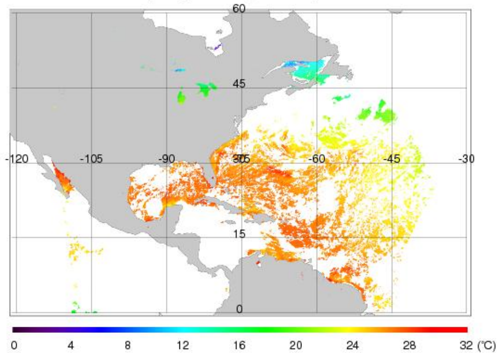
Figure 5.19: shows the SST from GOES-15 created by compositing three half hour daytime SST McIDAS Area files with an applied threshold of \geq 98\% clear sky probability.
