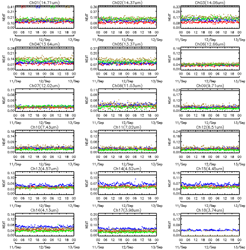
Figure 4.13: Diurnal variation of GOES-15 Sounder NEdT between 11 September 2010 and 12 September 2010. The solid line in each IR band plot is the specification value. The colors correspond to the 4 detectors.
