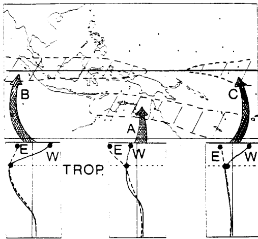
Fig. 4. Comparative QBO east-phase (E) and west-phase (W) representations of the basic differences in zonal wind profiles during the November-March portion of the annual cycle. Profiles are shown for areas near the equator in the far West Pacific (B) and near the Dateline (C), as well as off-the-equator in the SPCZ and in the Australian monsoon circulation (A). The "dots" on the profiles emphasize key differences in the vertical shear values between the upper troposphere and lower stratosphere.
